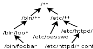
Figure 3: An example FCGlob tree.
